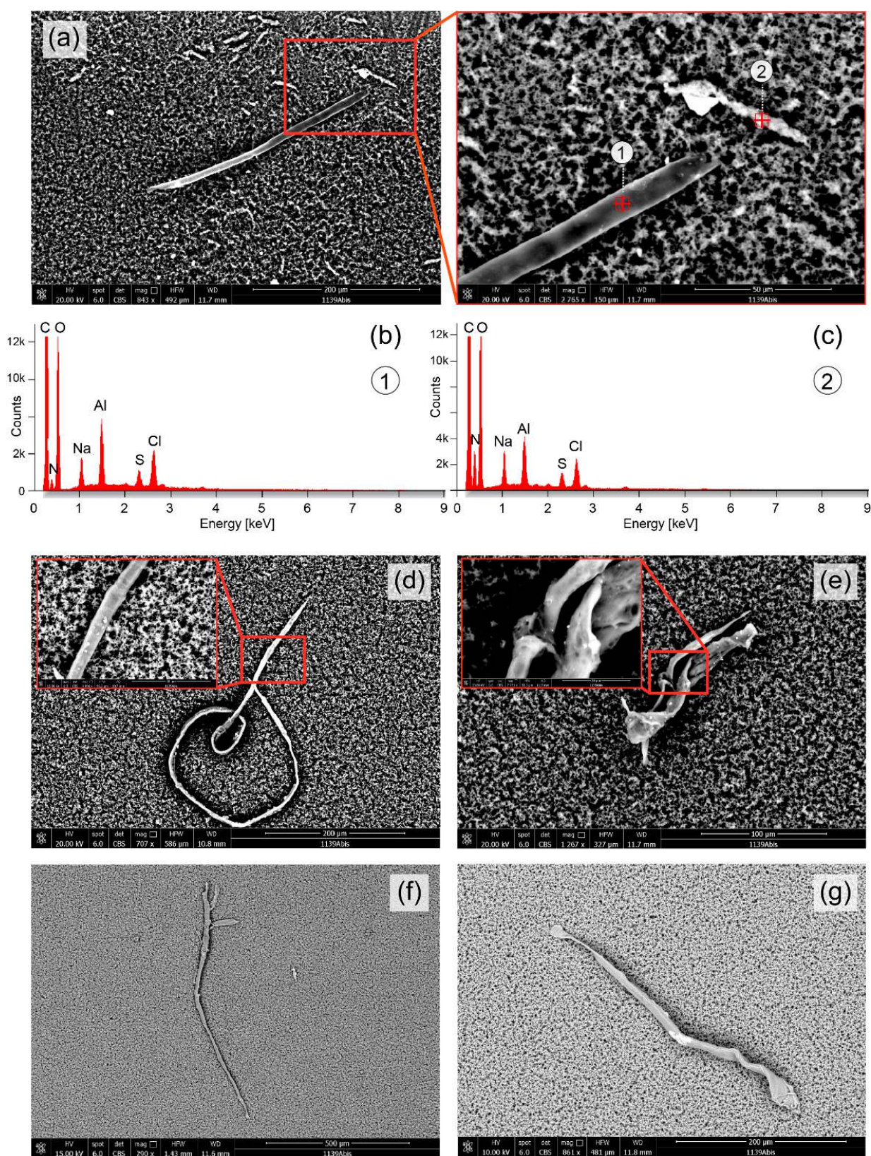
Figure 4. Elongated objects detected in the upper part (a,d,e) and middle part (f,g) of the vial with the eluate. (a) An object with a length of about 280 µm, diameter of about 9 µm, and a smaller particle nearby with a length of about 50 µm. Both objects consisted mainly of Al, Na, Cl and S (b,c). (d) Further elongated objects detected with lengths of about 925 µm (d), 140 µm (e), 850 µm (f) and 350 µm (g). In the objects shown in (d,e), nanoparticles are visible on their surface.
